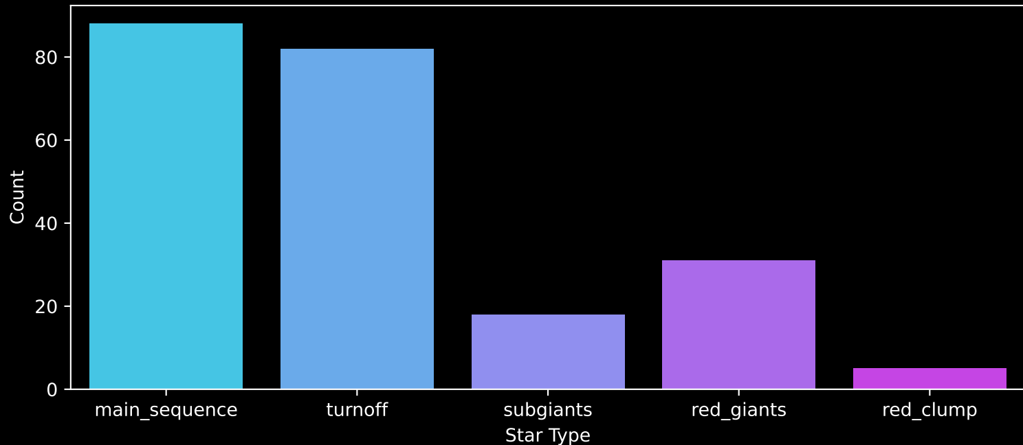
GALAH DR4 Field: [7218] Count plot of Star Type
