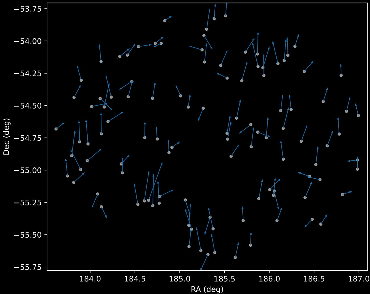
GALAH DR4 Cluster 0 Proper Motion Vectors (n=107)
