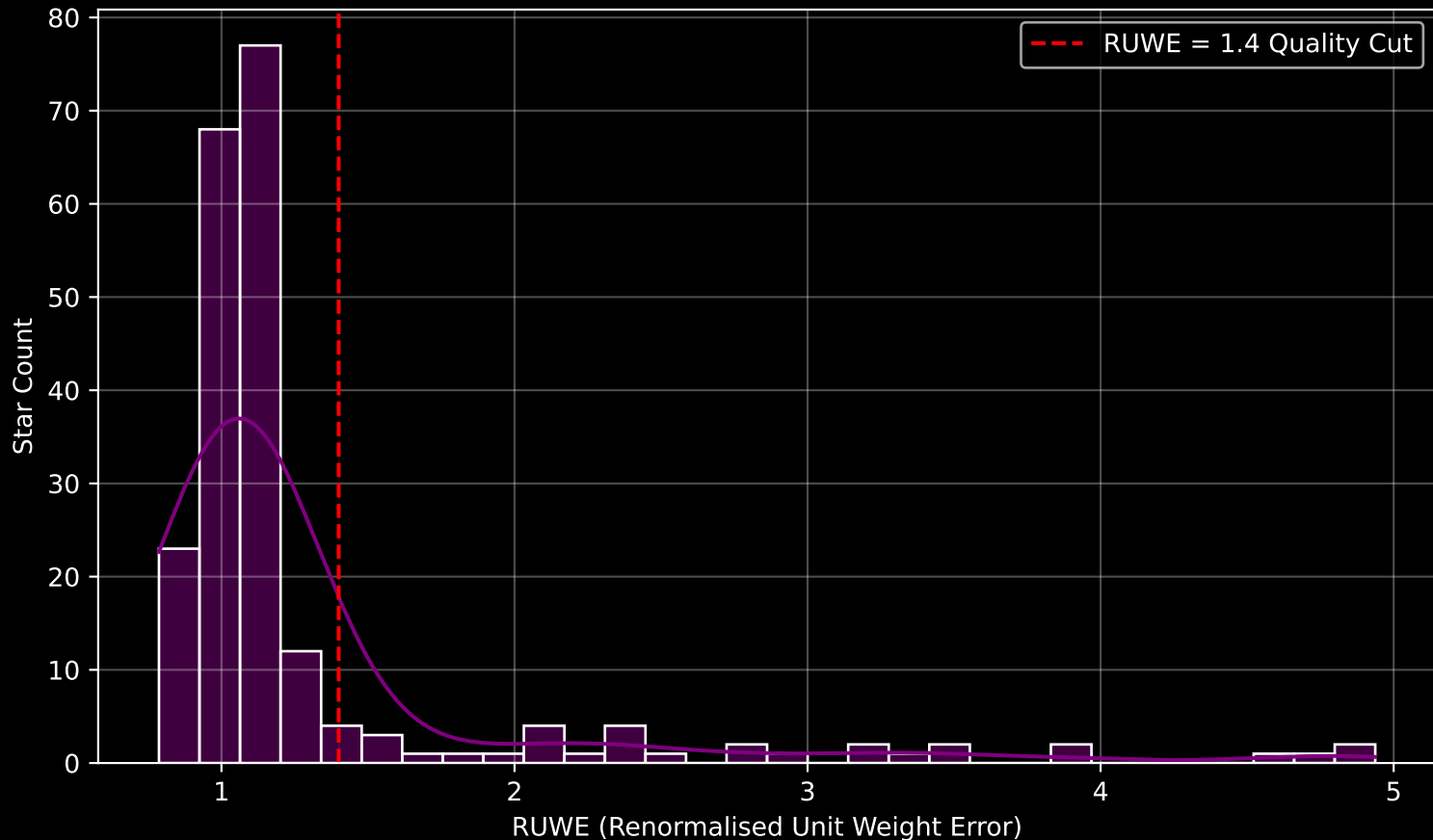
GALAH DR4 Field [7218] RUWE Distribution (n= 214)
