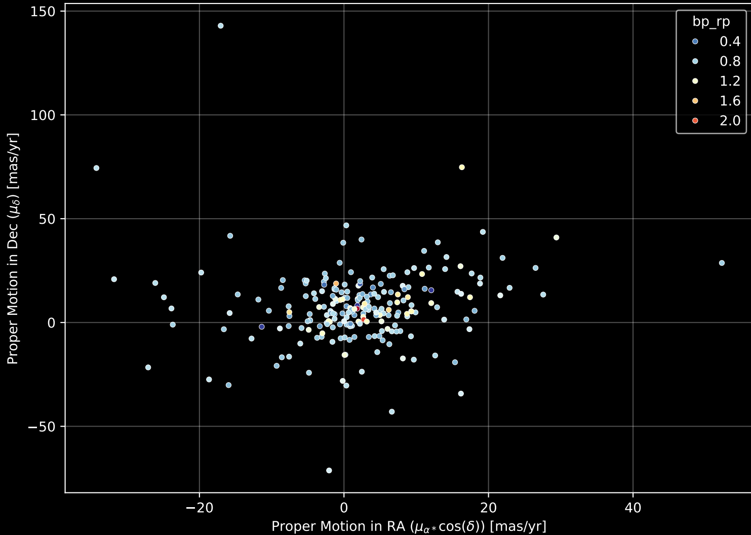
GALAH DR4 Field: [7218] Proper Motion Diagram (n= 224)
